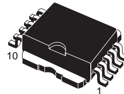
PowerSO-10™
